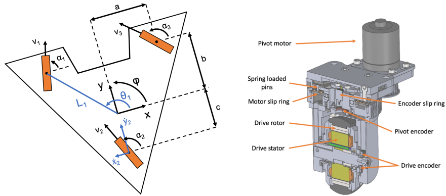
(a) Schematic representation of swerve drive platform. (b) Cross-section of a single wheelset.
