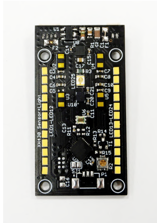
Fig. 5. Sensor board for the end effector.
