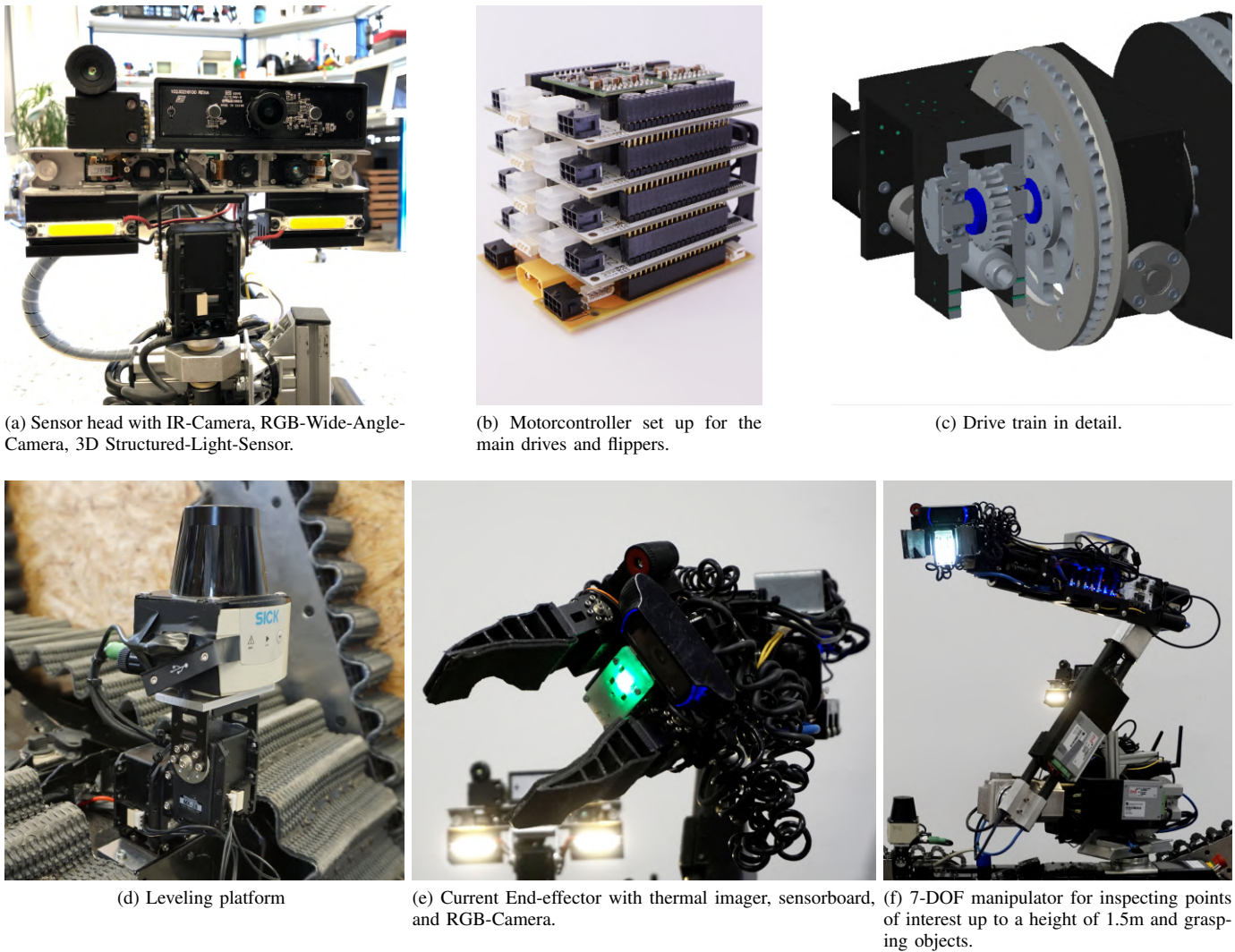
Fig. 6. Mechanical components and sensor concepts of Schroedi.
