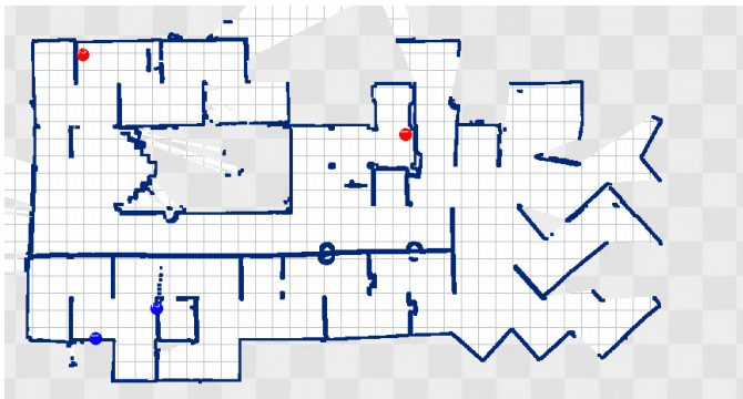
Fig. 8. Map generated by the ohm_TSD_slam
