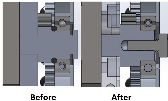
Fig. 7. Improvements to the wheel assembly
